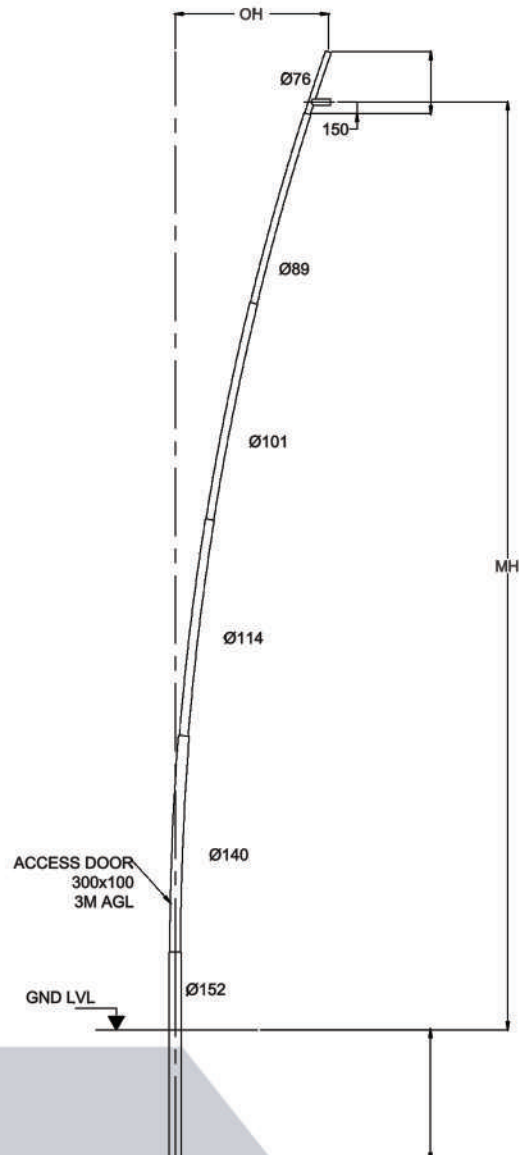
Curved Pole - 12m
