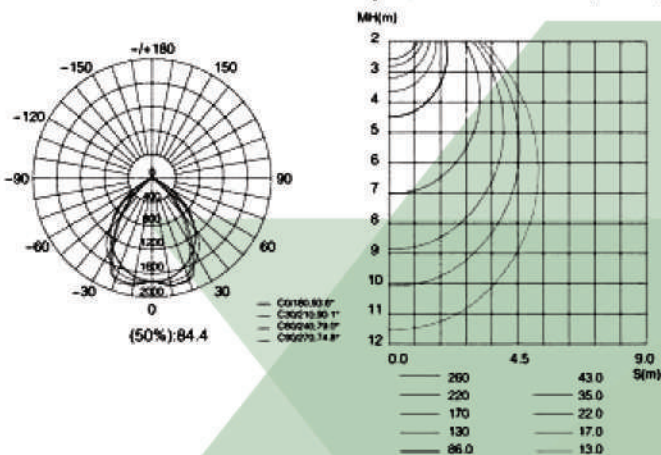
Space illumination curve (Unit: lx)
